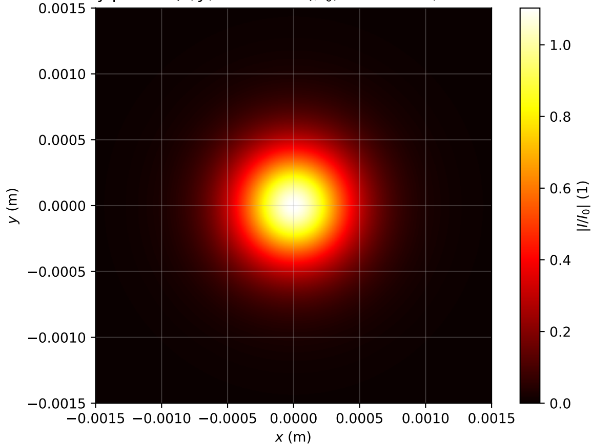
Intensity profile I(x, y, z = 1.990m)/I_0 , P_{in}=0.7P_{cr} , artificial time
